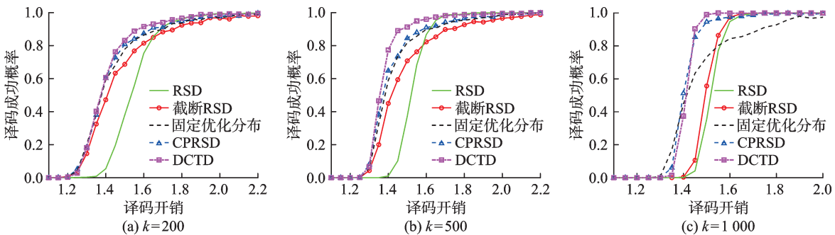
图4 不同度分布译码开销下的译码成功率 Fig.4 Successful decoding rate against overhead under different degree distributions
