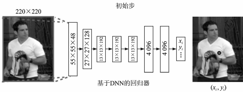
图 13 基于深度神经网络的姿态估计训练网络初始步 [41] Fig. 13 Initial pose estimation training stage based on CNN [41]
