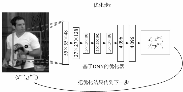
图 14 基于深度神经网络的姿态估计训练网络优化步 [41] Fig. 14 Pose estimation refining stage based on CNN [41]
