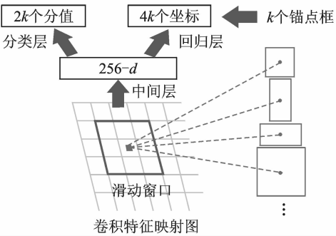
图 10 Region proposal network 结构 [34] Fig. 10 Region proposal network (RPN) [34]
