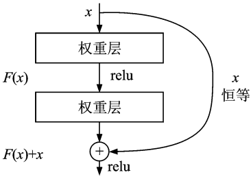
图 7 残差学习模块 [26] Fig. 7 Building block of residual learning [26]
