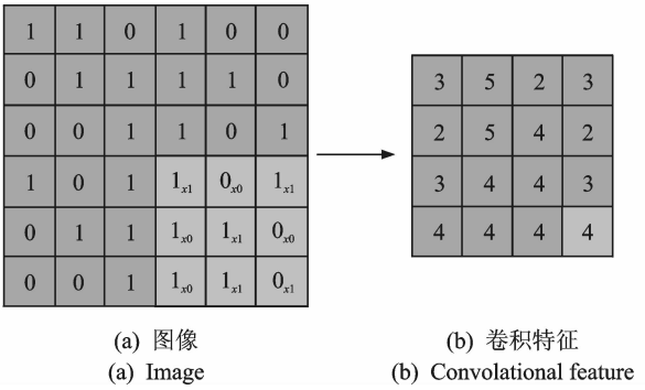
图 2 二维卷积运算操作示意图 Fig. 2 Illustration of two-dimensional convolution operation
