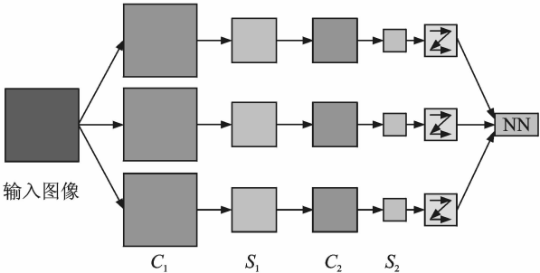
图 1 简化的卷积神经网络结构 Fig. 1 Simplified structure of convolutional neural network
