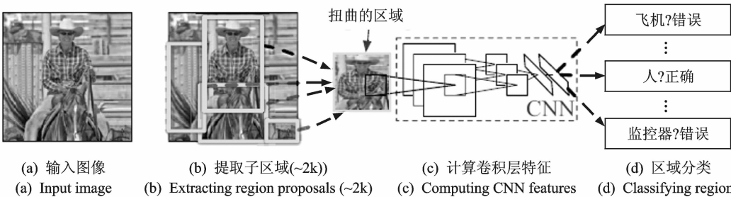
图 8 R-CNN 物体检测系统概览 [27] Fig. 8 Overview of R-CNN: Regions with CNN features [27]
