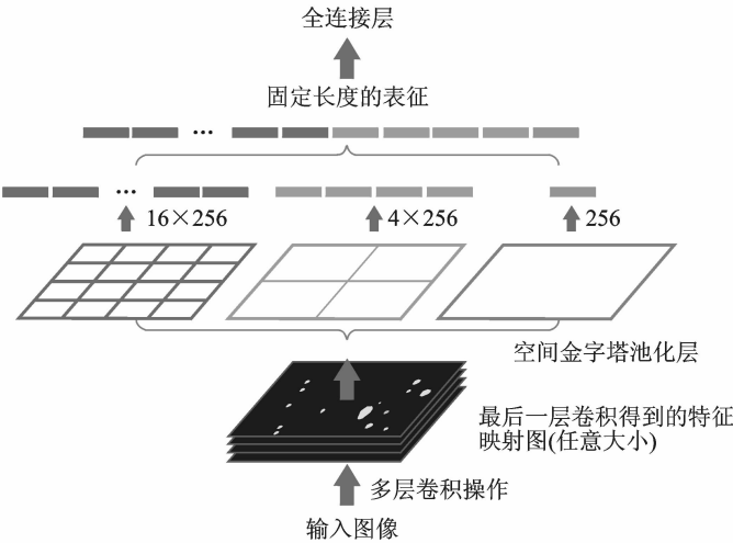
图 6 空间金字塔池化模型结构 [22] Fig. 6 Structure of spatial pyramid pooling model [22]
