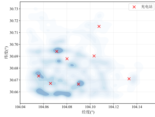
图 6 基于 FMPPSO 充电站选址方案 Fig.6 Layout Plan for FMPPSO Charging Station Site Selection
