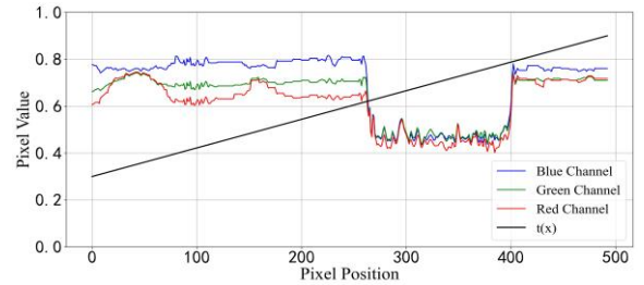
(a) Pixel value and transmittance of initial image
