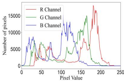
(b) Light dust image and its histogram
