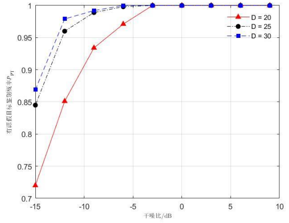
(b) False target identification probability
