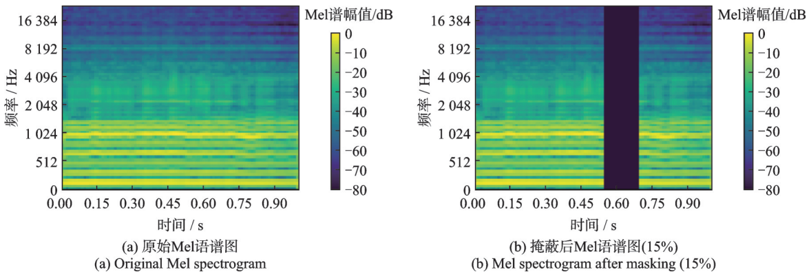
图3 以Mel语谱图为例的块状掩蔽策略 Fig.3 Block masking strategy with Mel spectrogram as an example
