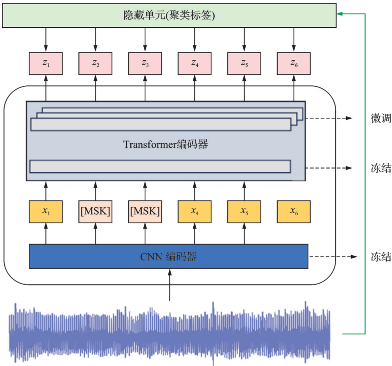
图2 HuBERT 自监督语音特征提取模型结构 Fig.2 Architecture of the HuBERT self-supervised speech feature extraction model
