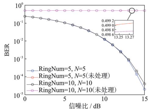
图6 双模块干扰消除方案处理与未处理的BER比较图 Fig.6 BER comparison between dual-module interference cancellation scheme and untreated scenario
